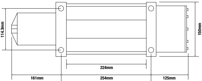
BOLTING PATTERN
